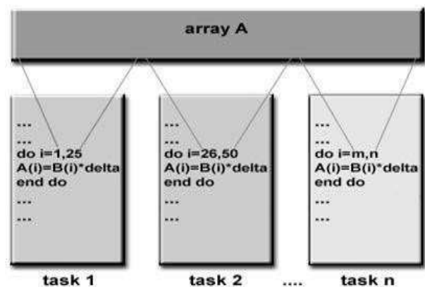
Figure 1 data parallel model
