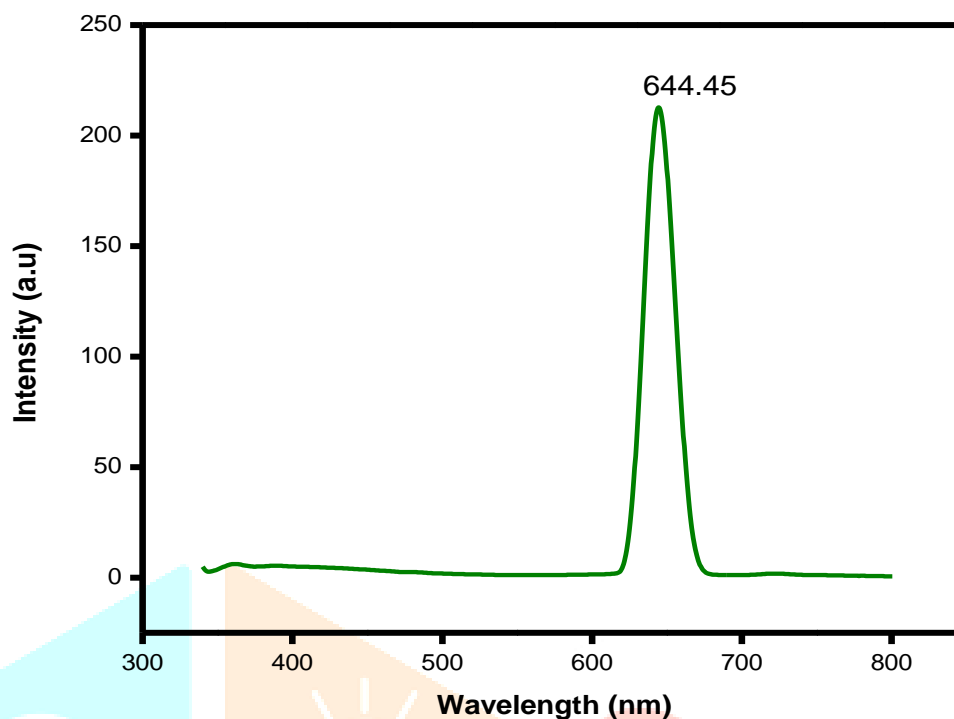
Figure 6: Photoluminescence Spectrum of ZnO nanoparticles
