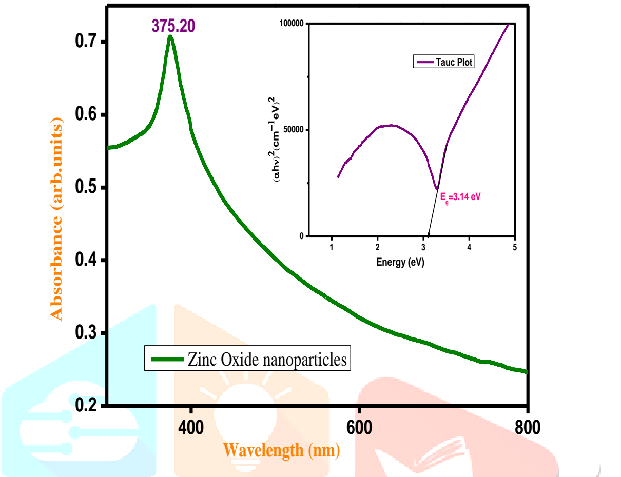
Figure 3: UV-Visible absorption spectrum of Zinc Oxide nanoparticle using Morinda citrifolia leaf extract
