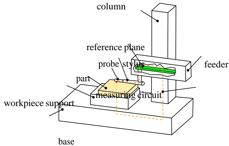
Figure 2. Components of a skidless measurement system; modified from [6,9].
