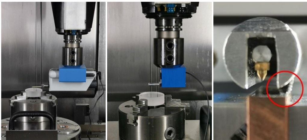
Figure 3. Skidless touch probes: (left) SD26 from MAHR and (middle) MiniProfilier from Breitmeier; (right) support on workpiece of MiniProfilier.
