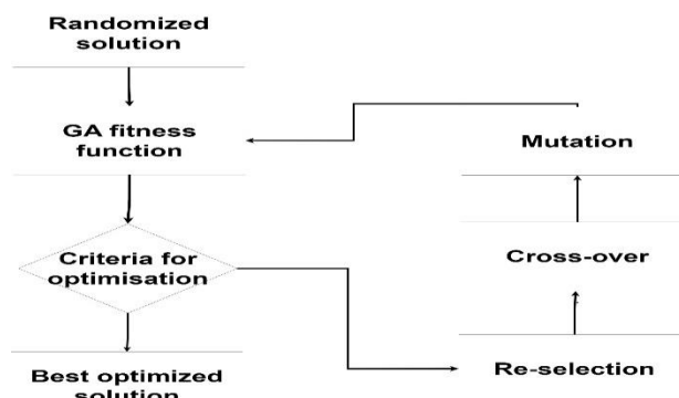
Figure. 3. Flow chart of the Genetic algorithm
