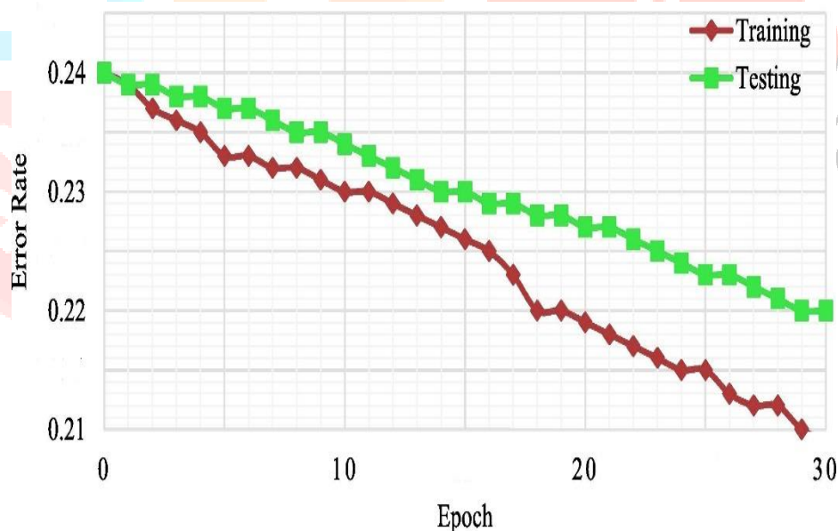
Fig. 7 Proposed model error rate plot
