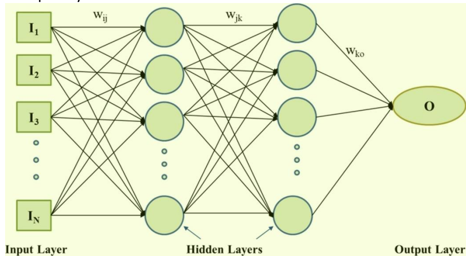
Fig. 2 Structure of the ANN
