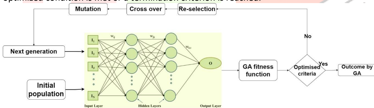
Fig. 4 Proposed ANN model with GA for yield prediction
