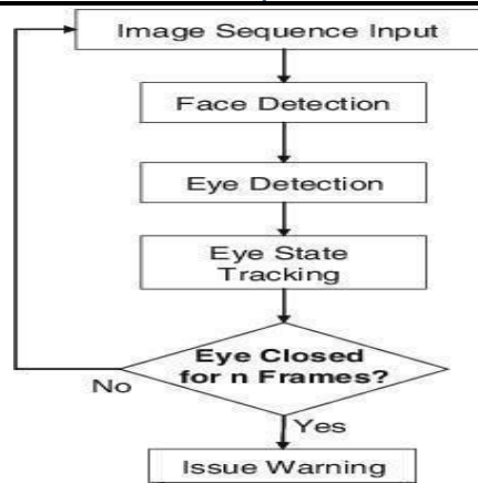
Fig. 2 Drowsiness Detection System Model
