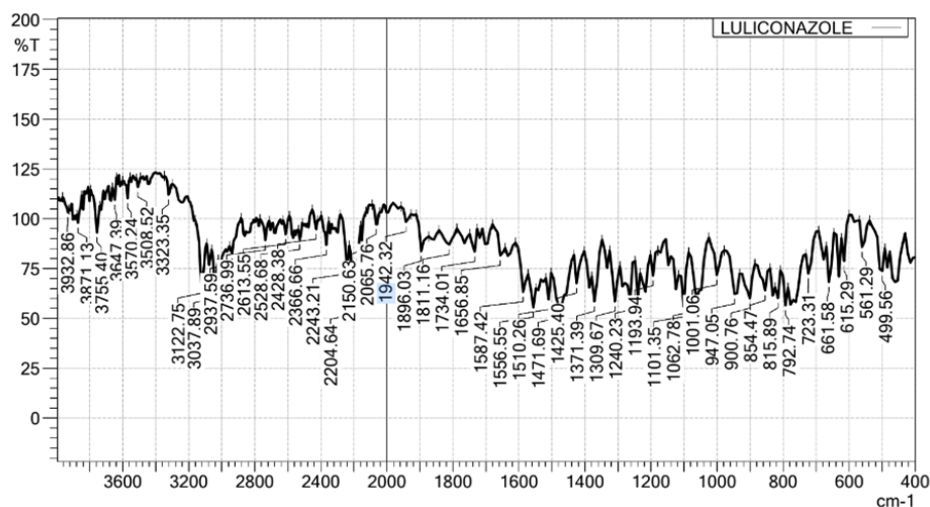
Graph No 2. FTIR Spectrum of Luliconazole
