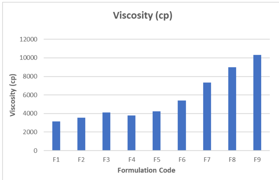
Graph No 7: - Comparison of Viscosity of factorial batches
