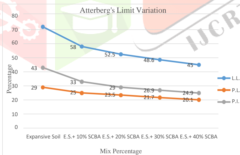
Fig.1 Atterberg's Limit Variation
