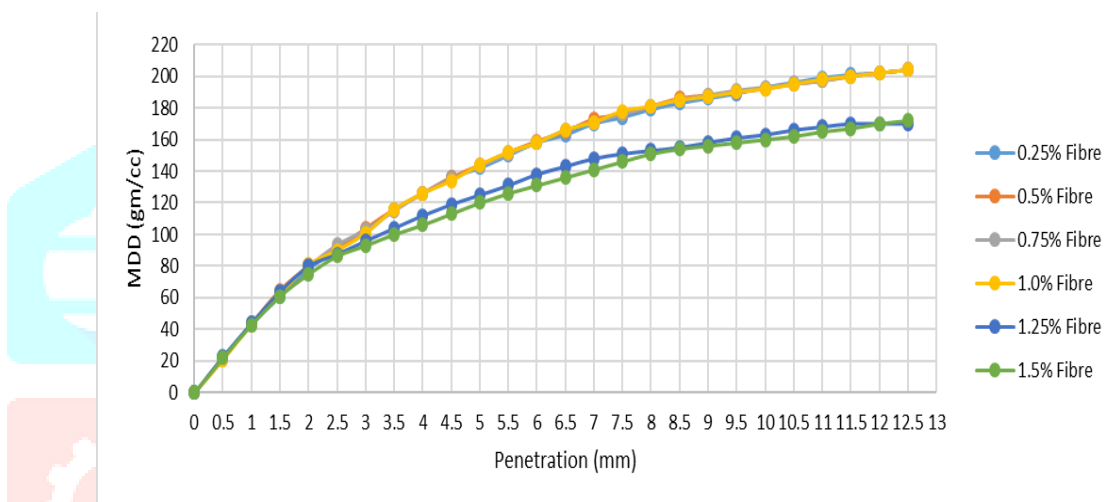
Fig. 6 – CBR for mix specimen of 20% SCBA and Expansive Soil with Fibre (AR – 80)
