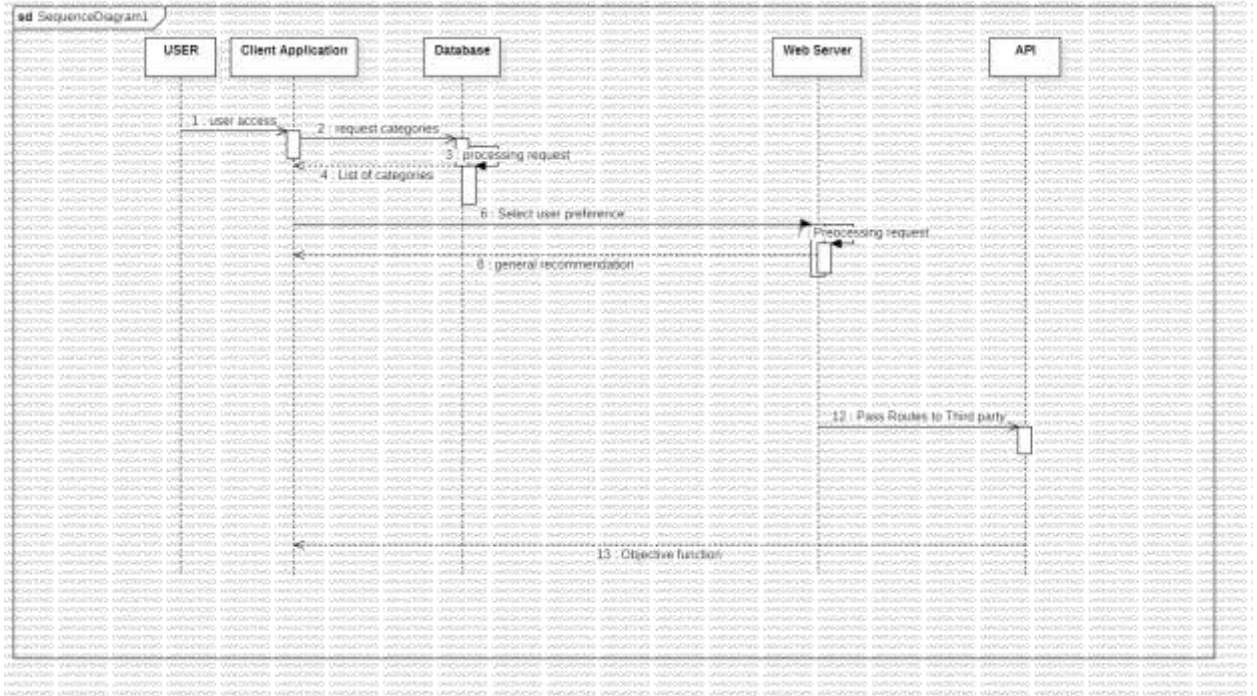
SEQUENCE DIAGRAM
