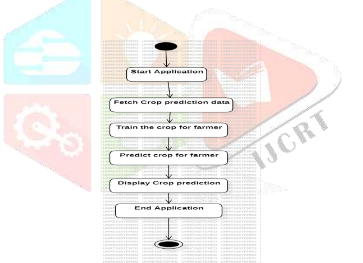
ACTIVITY DIAGRAM
