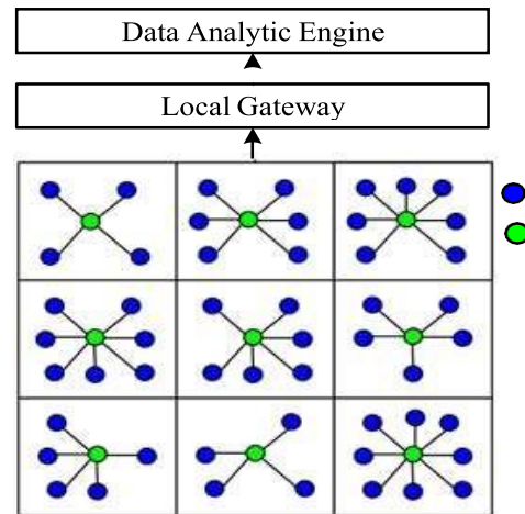
Fig. 2. Generalized Architecture 4S-UEM
