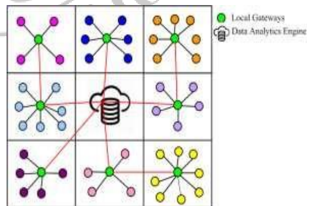
Fig.5.Selection of Local Gateway ( L_g ) in the Urban Cluster of 4S-UEM Fig 6.The Transmission Process of Messages from uC through L_g to DaE of 4S-UEM.
