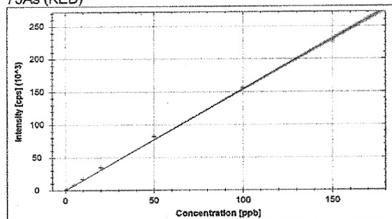
75As (KED)
