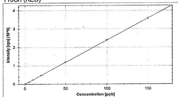
118Sn (KED)
