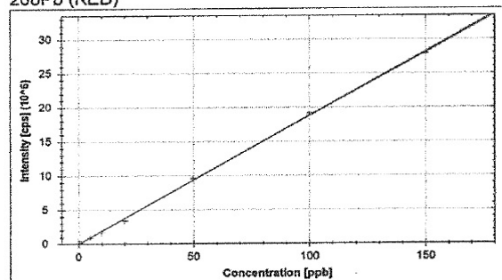
208Pb (KED)
