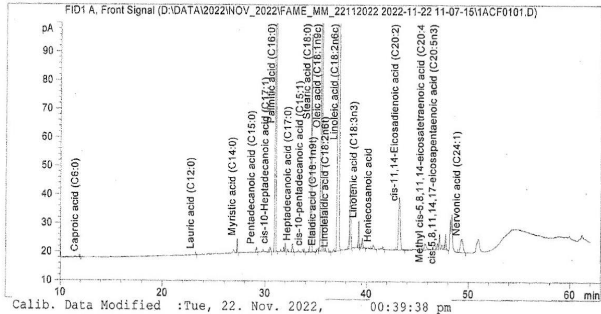
Figuer-1. Chromatogram of the 37 Component FAME mix obtained using the Varian GC-FID equipment
