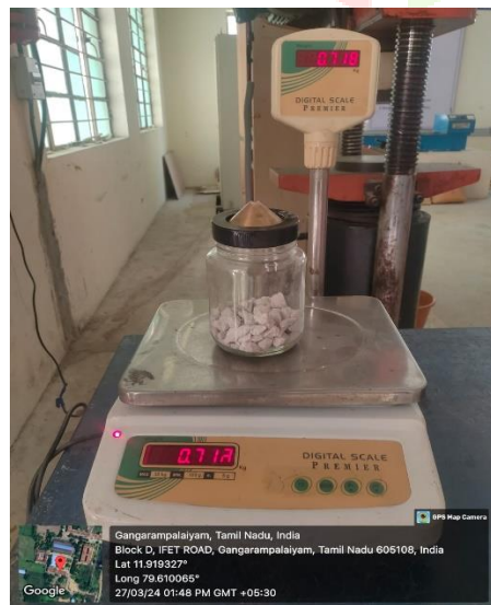
Fig 5.5 SPECIFIC GRAVITY OF PUMICE STONE
