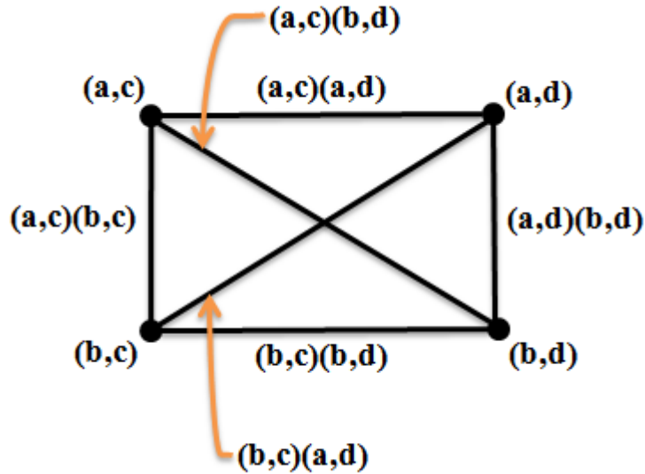
Figure 2 G_1 \oplus G_2
