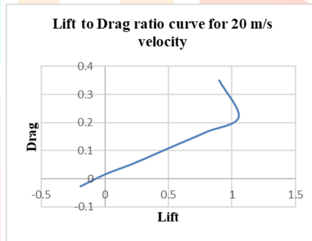
Fig.2.4 Lift to drag ratio curve
