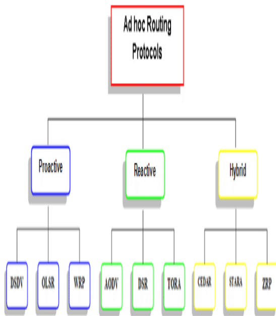
Fig.1. Classification of Routing Protocols
