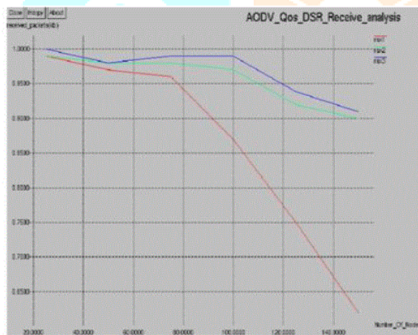
Fig 5: Received Ratio of DSR, AODV and DSDV
