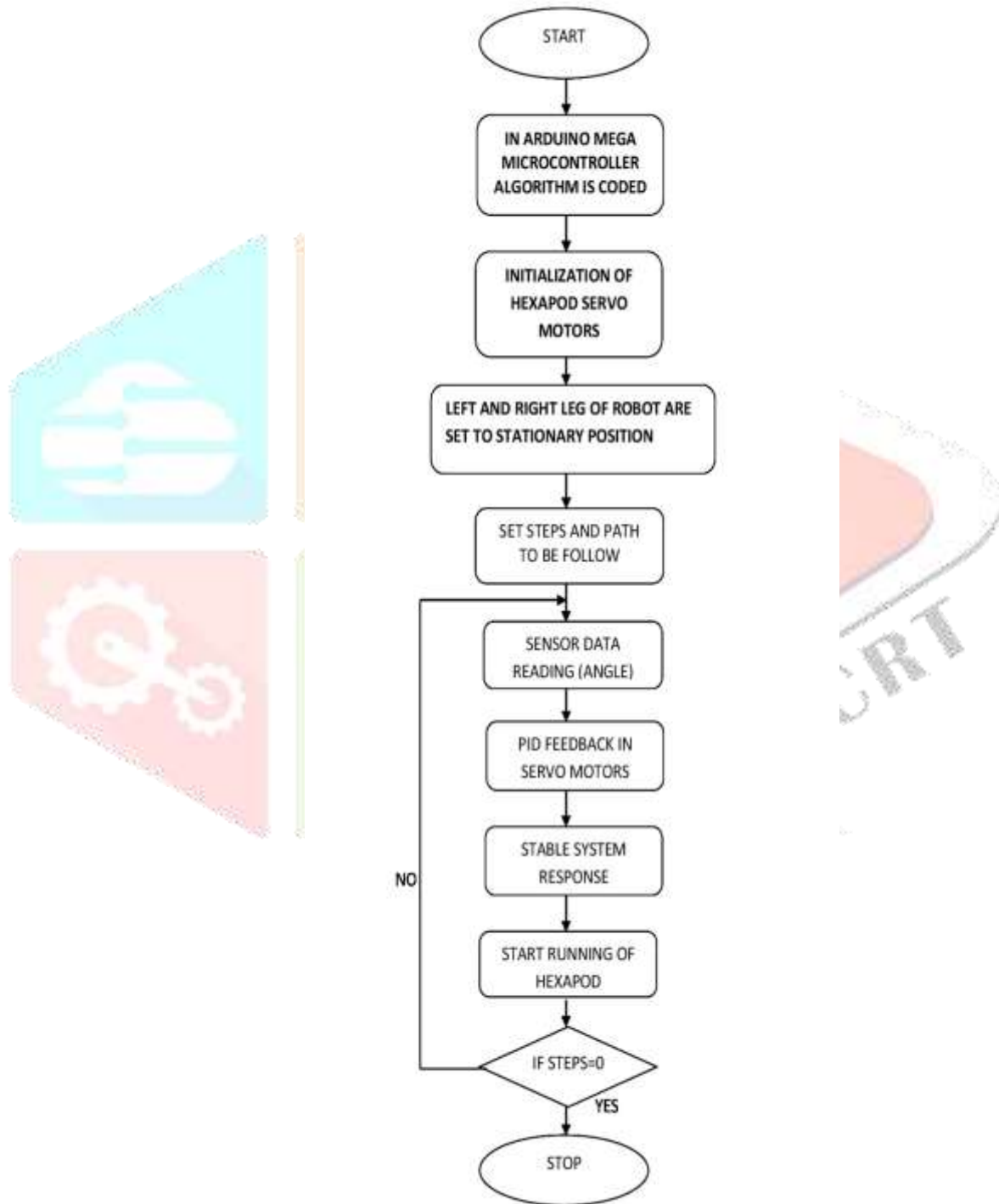
Fig 3: Flowchart of a system
