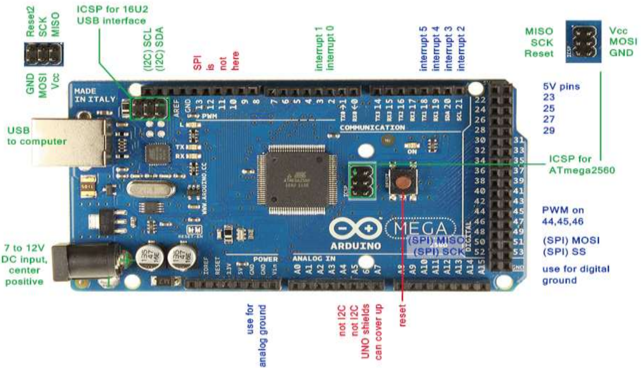
Fig 4: Arduino Atmega2560
