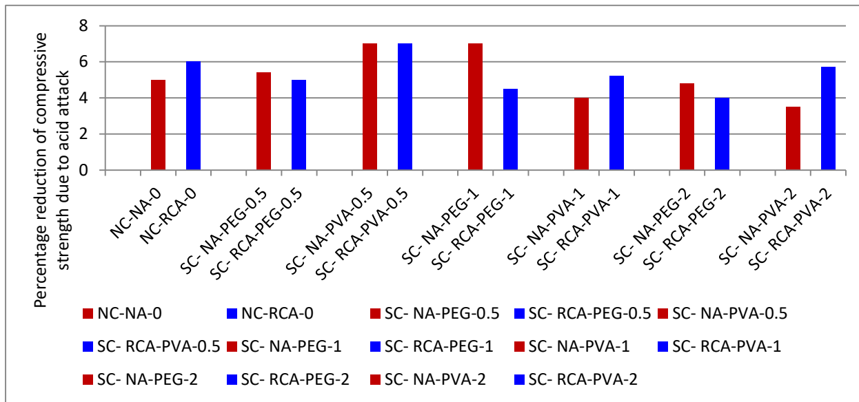
Figure: 5 Comparison of Percentage reduction due to acid attack of SC-NA with SC-RCA using PEG-600 and PVA
