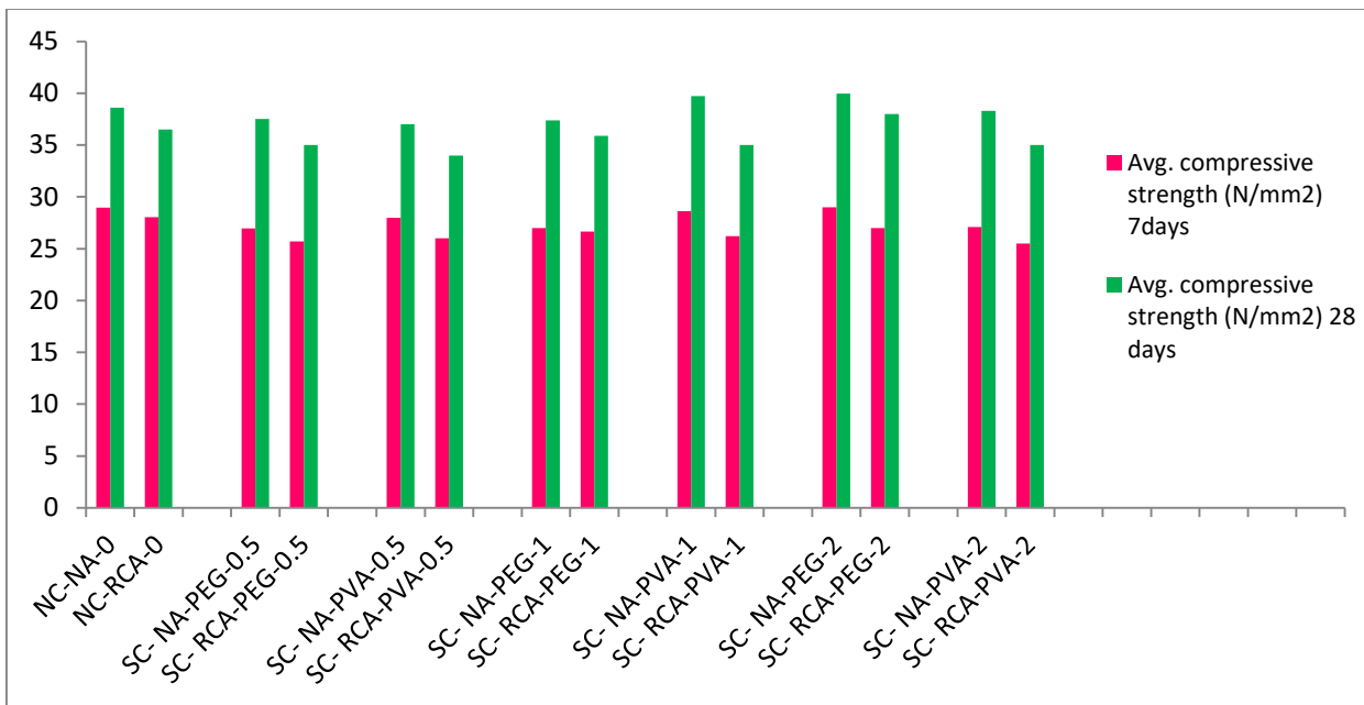
Figure:2 Comparison of compressive strength of SC-NA with SC-RCA using PEG-600 and PVA
