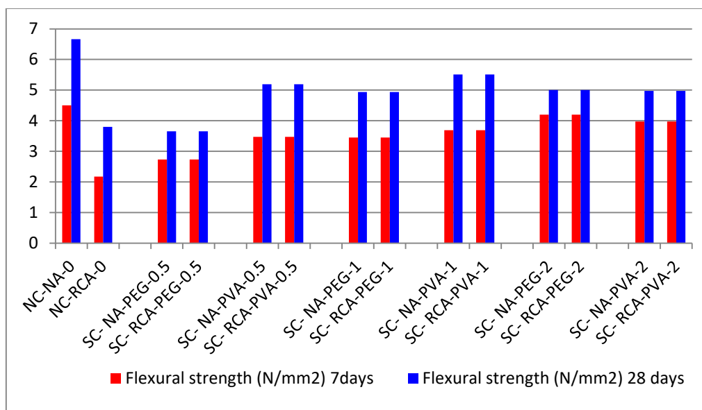
Figure: 4 Comparison of Flexural strength of SC-NA with SC-RCA using PEG-600 and PVA
