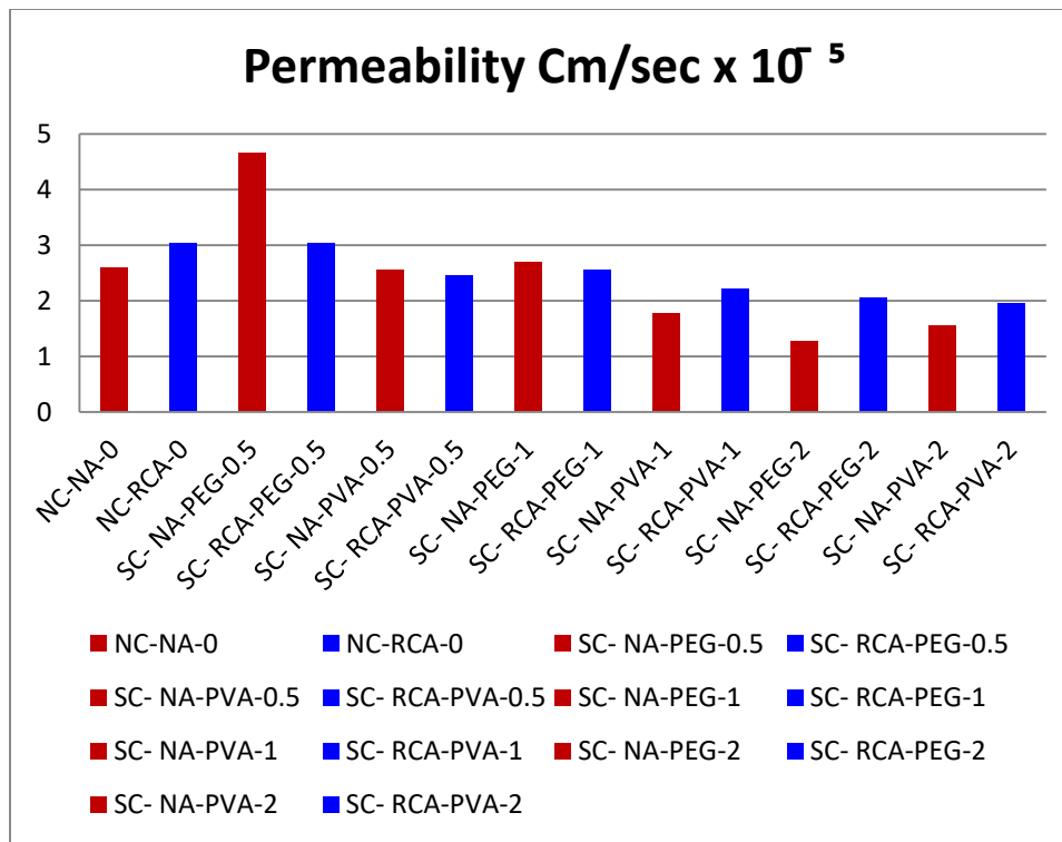
Figure: 7 Comparison of permeability of SC-NA with SC-RCA using PEG-600 and PVA
