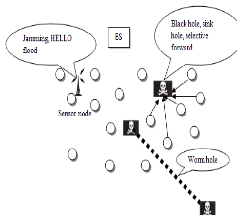
Figure 2: Routing attacks in WSN
