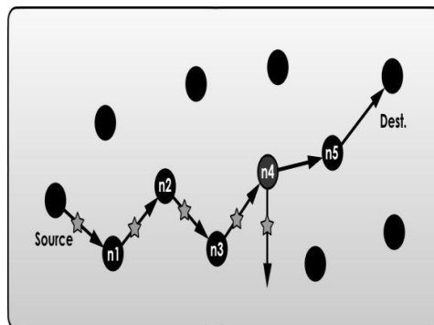
Figure 4: Selective Forwarding in WSNs
