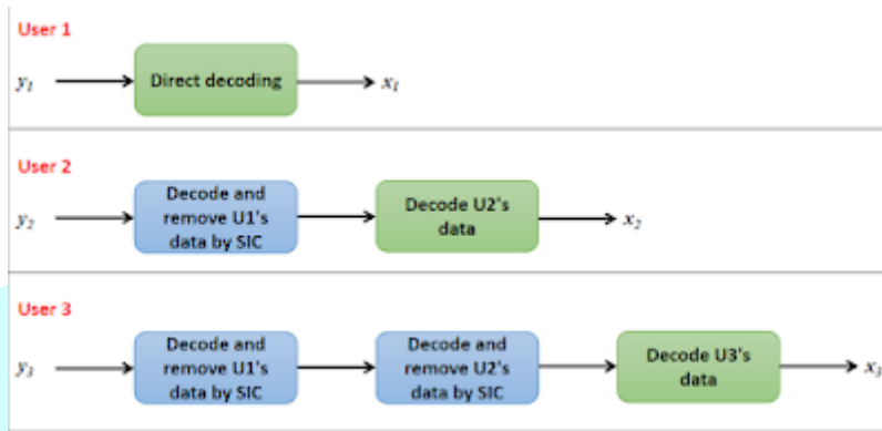
Figure 4: Attack decryption procedure
