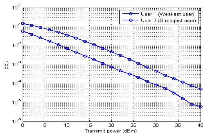
Figure 9: BER v/s Transmit power RSMA 2 user
