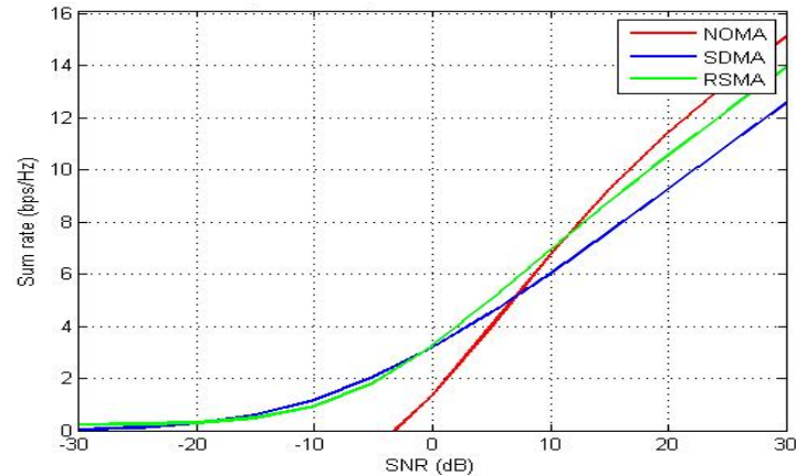
Figure 11: Comparison study of SDMA, NOMA, RSMA
