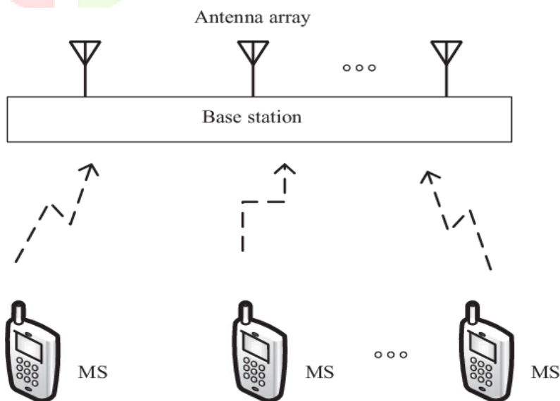
Figure 1: SDMA system Block Diagram
