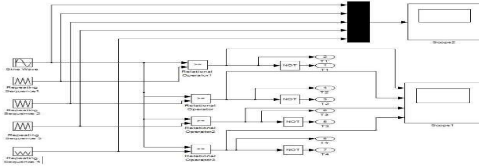
Fig.5. Firing circuit
