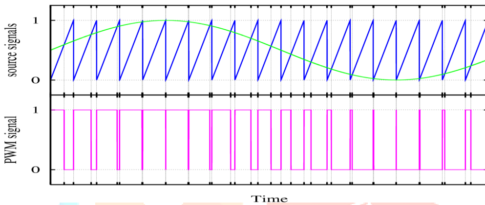
Fig.6. PWM waveform
