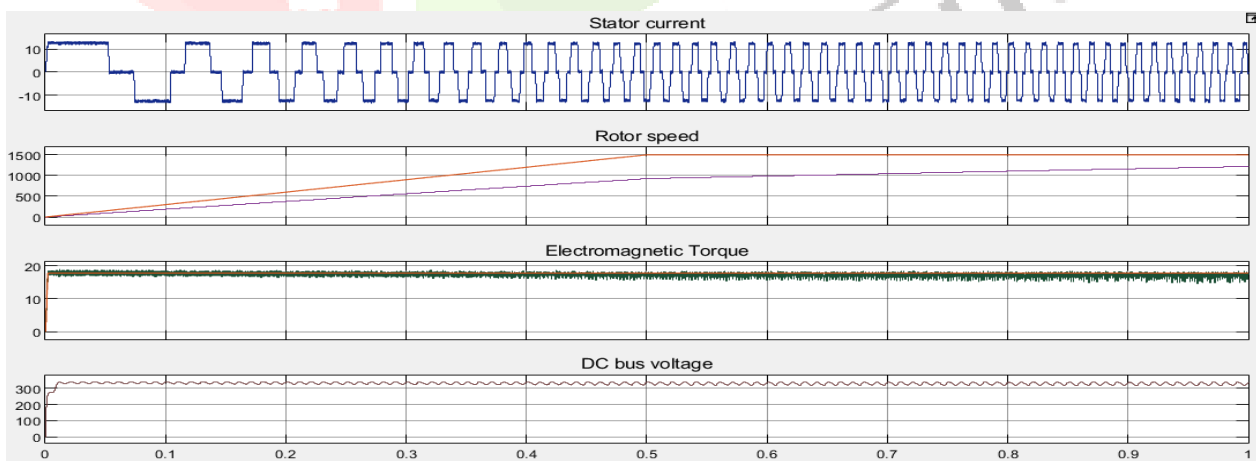
Fig.7.BLDC drive characteristics
