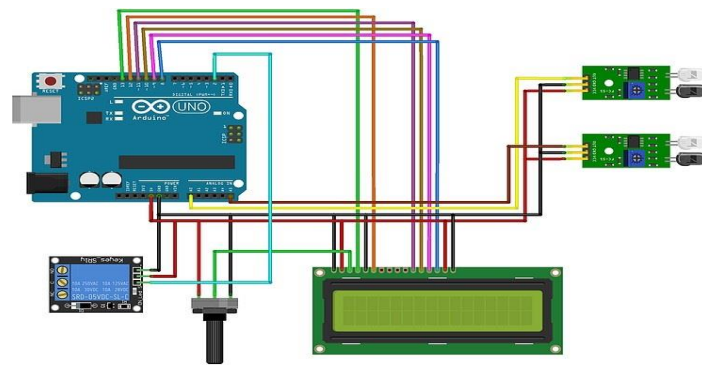
Fig. 1.1 Visitor counter
