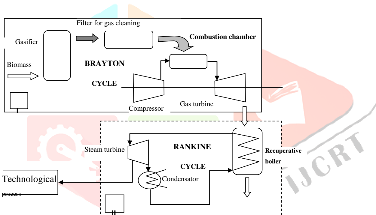
Figure 2.5: Biomass/Integrated Gasifier/Gas Turbine Combined Cycle.
