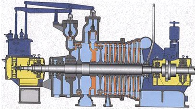
Figure: 2.4: Extraction Condensing Steam Turbine
