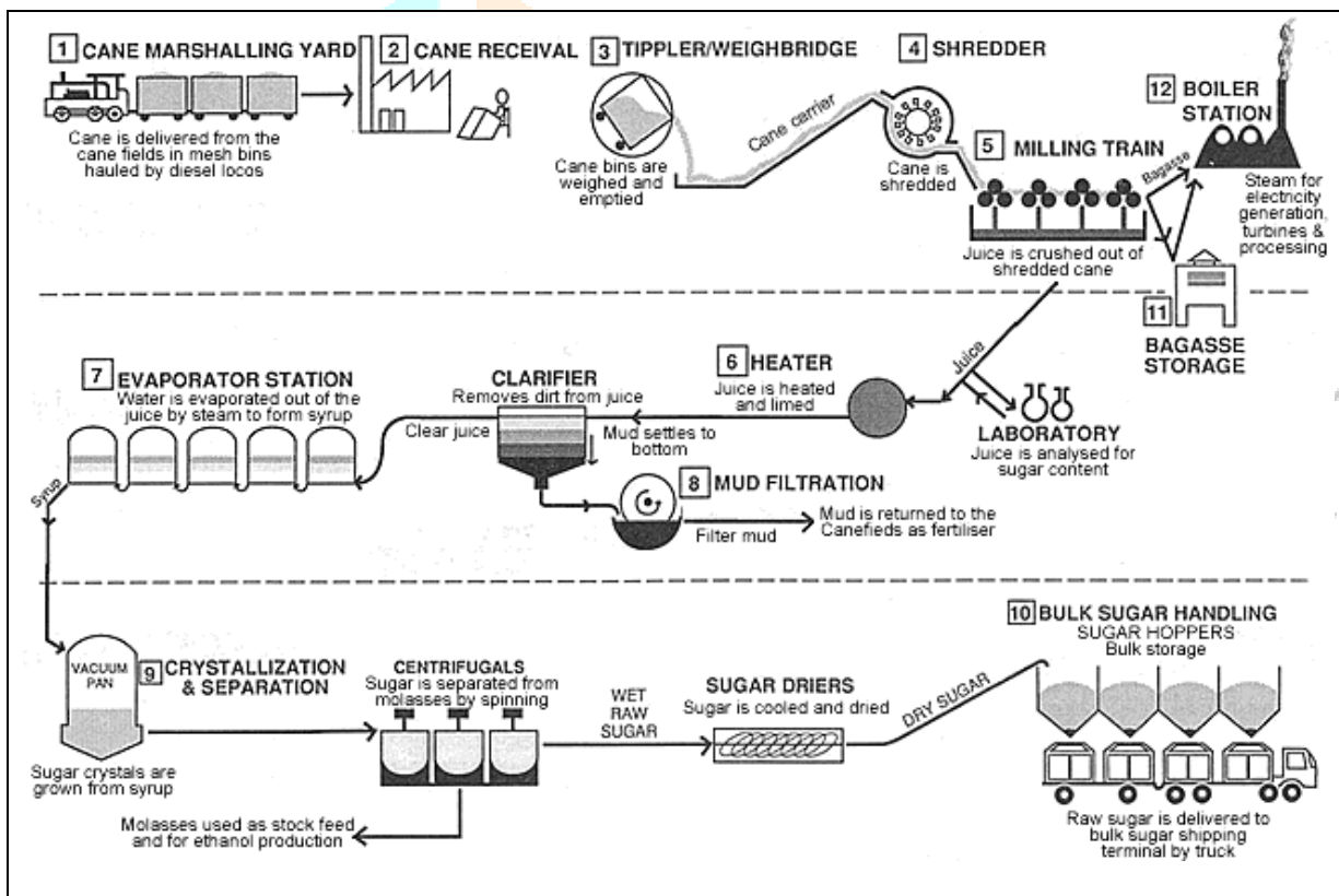
Figure 2.2: Simplified Diagrammatical Explanation of the Process for Producing raw sugar
