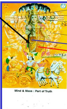
Fig. Divine Mechanics Unit Mind – CCP, CP and information s – Code PcPs with B-Bit – Mass
