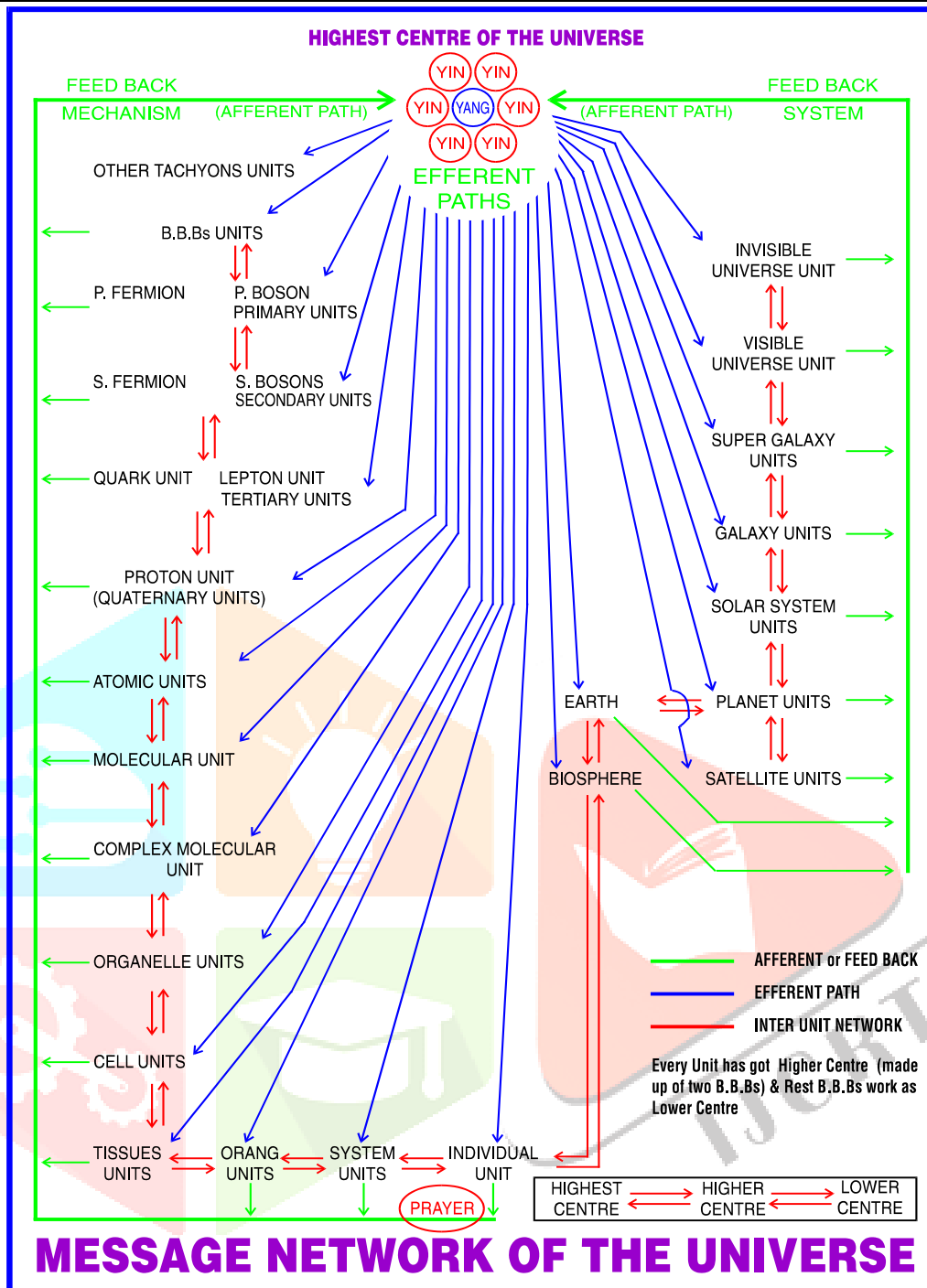
Fig. 8 Messages Net work of the Universe
