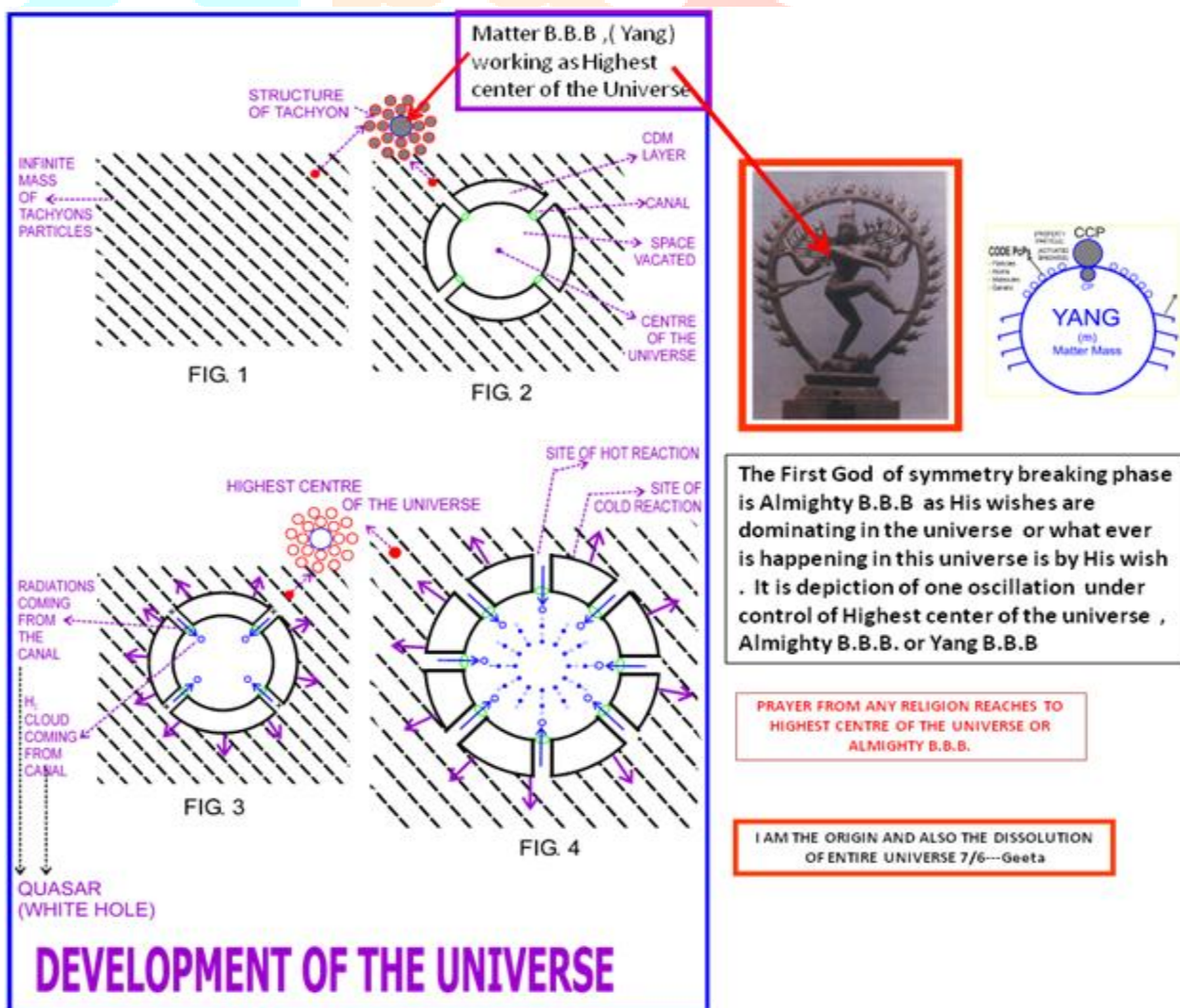
Figure Hoyle Narlikar Universe OR Universe “T”
