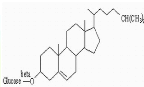
Figure 1. Structure of charantin.
