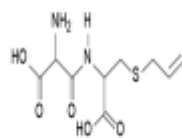
γ-glutamyl-S-allyl-L-cysteine
