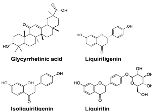
Fig. 1. Chemical structures of four compounds (glycyrrhetic acid, liquiritigenin, isoliquiritigenin, and liquiritin).
