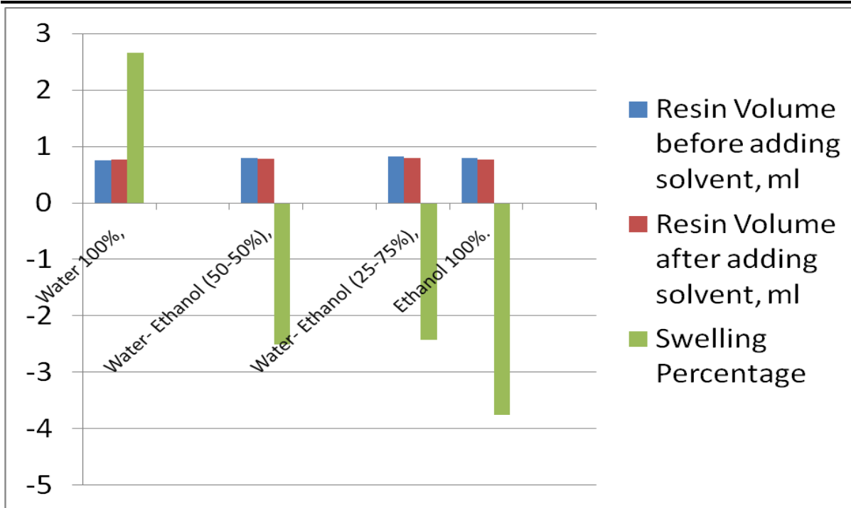
Fig 1: Comparison of swelling characteristics ZrPthAs in Water- Ethanol medium
