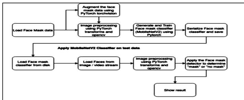
Figure 2. Represent the Architecture of Proposed Model
