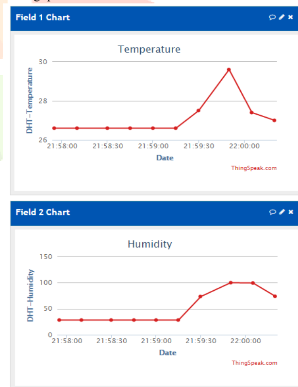
Fig 1 Thingspeak channels
