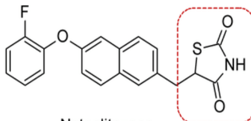
Netoglitazone
