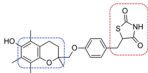
Troglitazone
