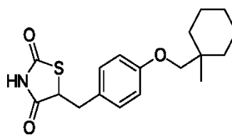
Ciglitazone
