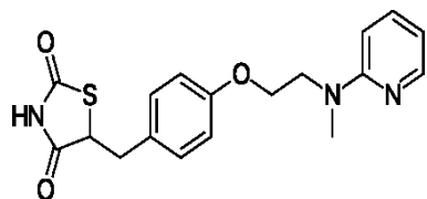
Rosiglitazone
