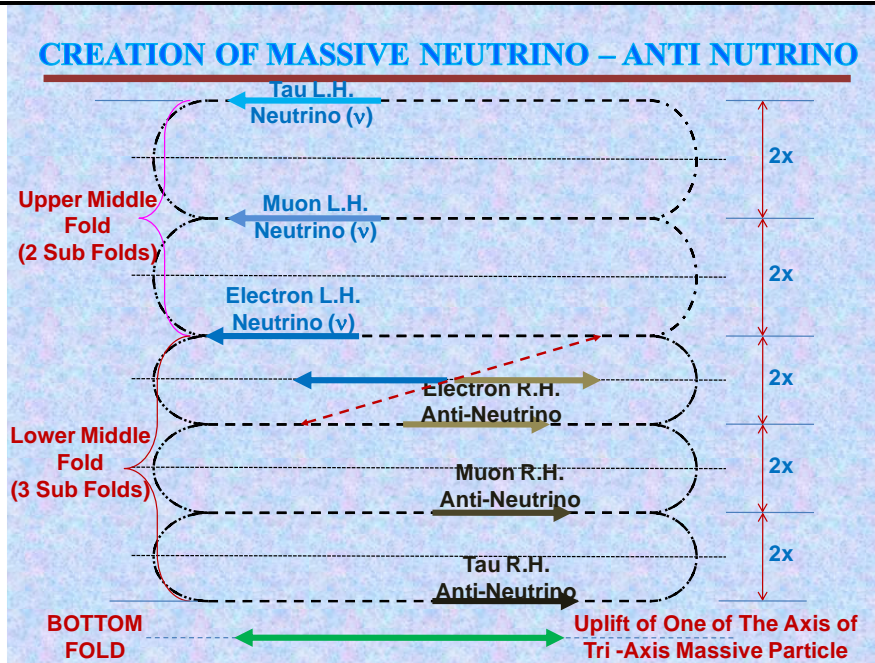
Fig. 12: Creation of Pair of Massive Neutrinos and Antineutrinos
