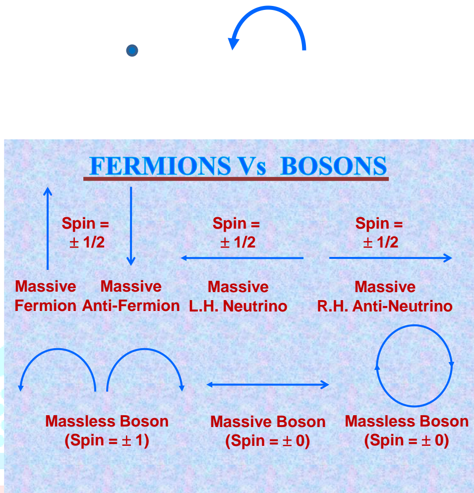
Fig. 3: Massive Fermions Vs Massless Bosons
