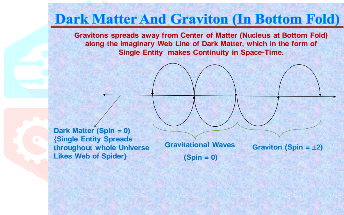
Fig. 8: Dark Matter (Single Entity Like Web of Spider) And Gravitational Waves (Spin= 0)
