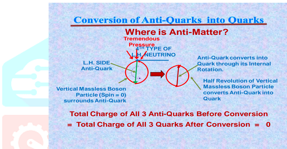
Fig. 7: Conversion of Anti-Quarks (Anti-Matter) into Quarks (Matter)
