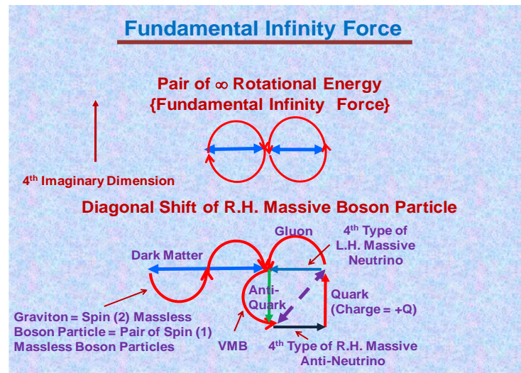
Fig. 14: Infinity ( \infty ) Like Rotation of Massless Boson (Spin=0) Particles at TeV Range
