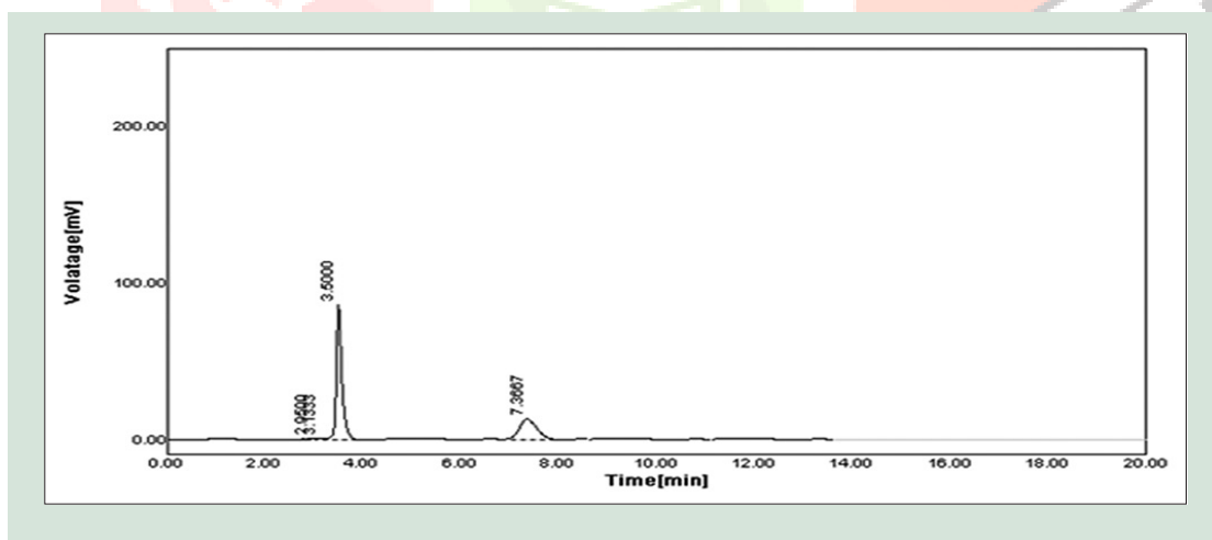
Figure 6: Chromatogram of abacavir and lamivudine in tablet formulation
