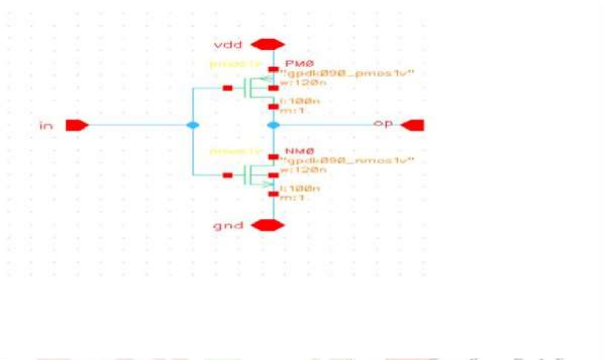
Fig.13 (Inverter Schematic Diagram)
