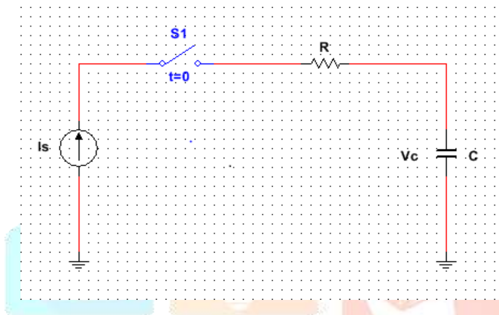
Fig.3 (Equivalent circuit to determine the losses by adiabatically loading a capacitance)
