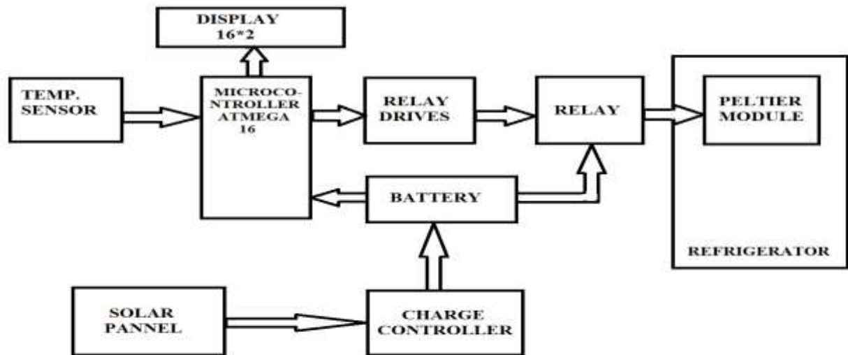
Figure. Block diagram solar based refrigeration system
