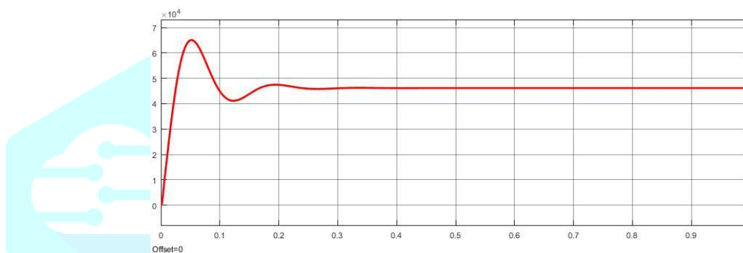
Fig. 4. Speed Response of simulation model of DC motor speed control without approximation
