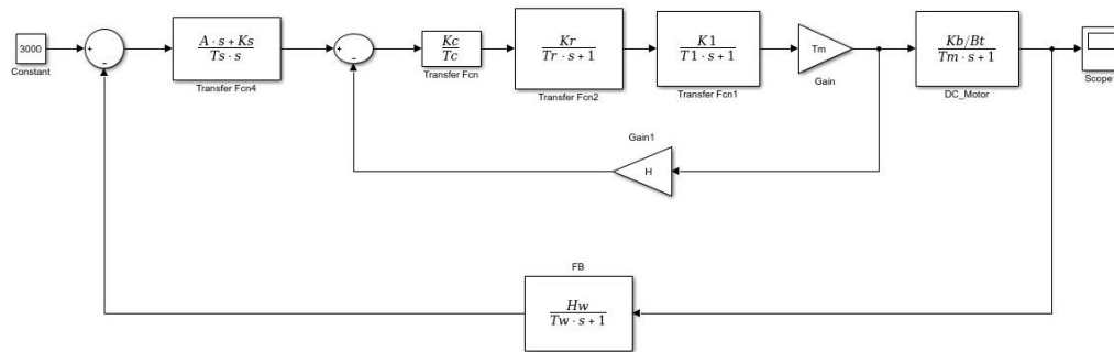
Fig.3. Simulation of DC motor speed control with approximation
