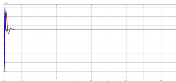
Fig.6. Comparison of Speed Response of both simulation models
