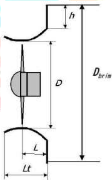
Figure : 2 Shape of Wind Lense
