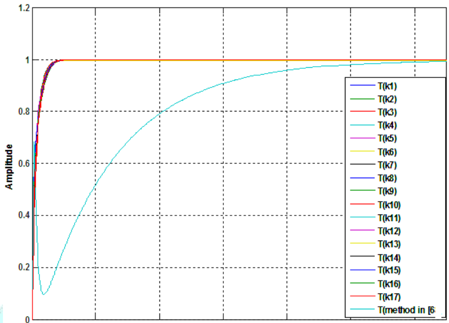
Figure 4: Step response of YK controllers designed with MODA and method developed in [6]
