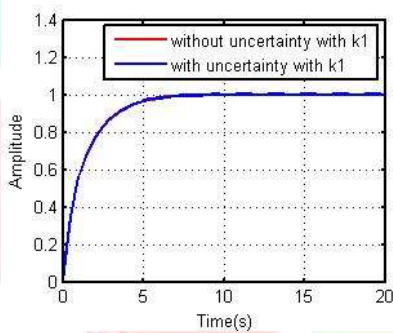
Figure 5: Step response of the plant using k_1 with and without uncertainty
