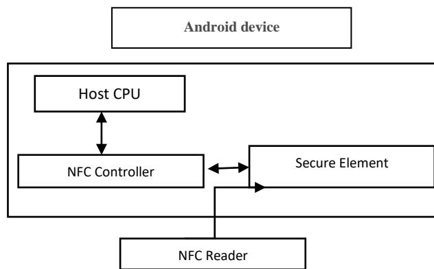
Figure 4: Card Emulation with a secure element
