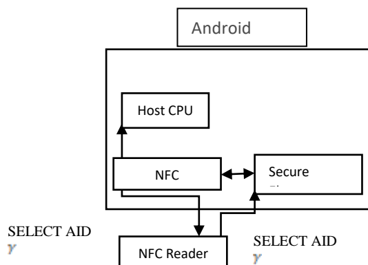
Figure 6: Device operating both SE and HCE
