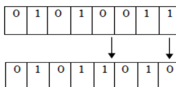
Figure 8: Mutation
