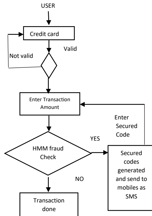
Figure 9: Proposed model of credit card fraud detection after training during detection
