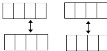
Figure 7: Crossover
