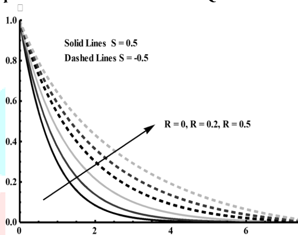
Figure 9: Variation of temperature profile for different values of R
