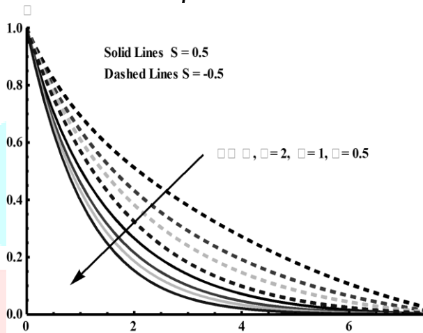
Figure 3: Variation of temperature profile for different values of \beta
