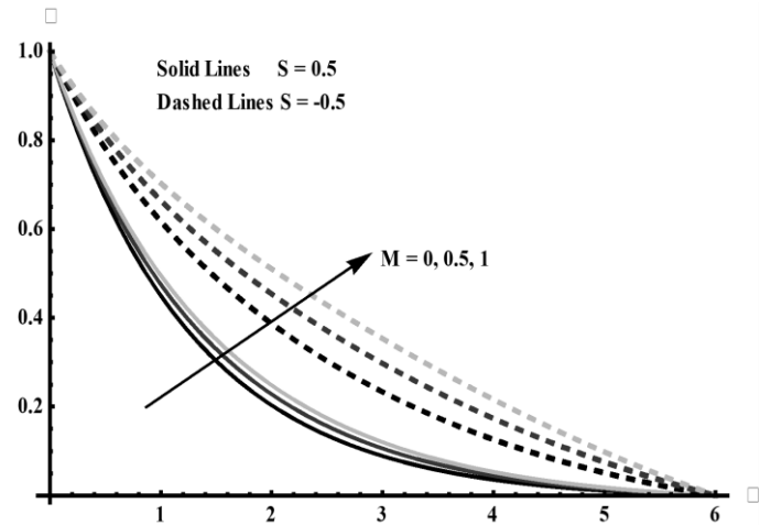
Figure 5: Variation of temperature profile for different values of M
