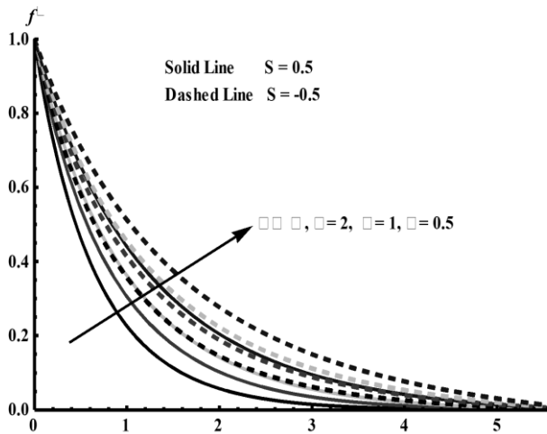
Figure 2: Variation of velocity profile for different values of \beta
