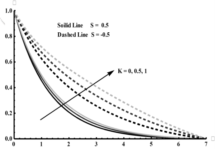
Figure 7: Variation of temperature profile for different values of K
