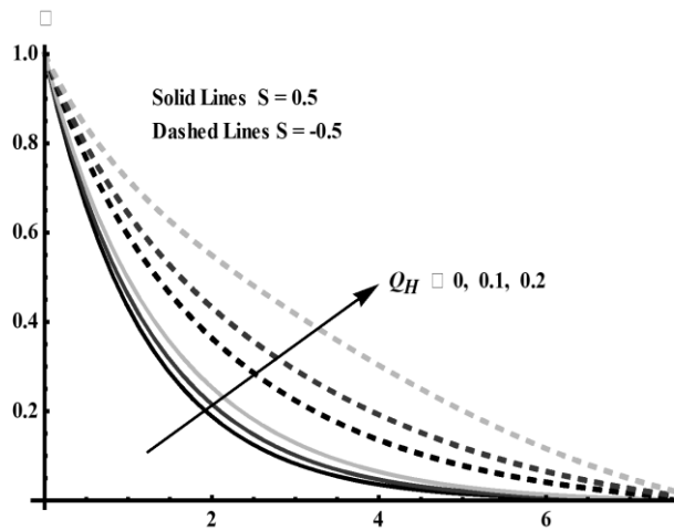
Figure 8: Variation of temperature profile for different values of Q_H
