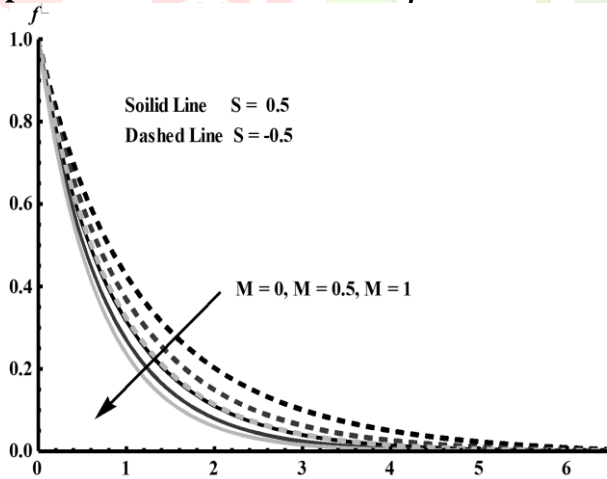
Figure 4: Variation of velocity for different values of M
