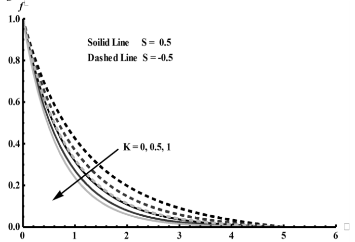
Figure 6: Variation of velocity for different values of K
