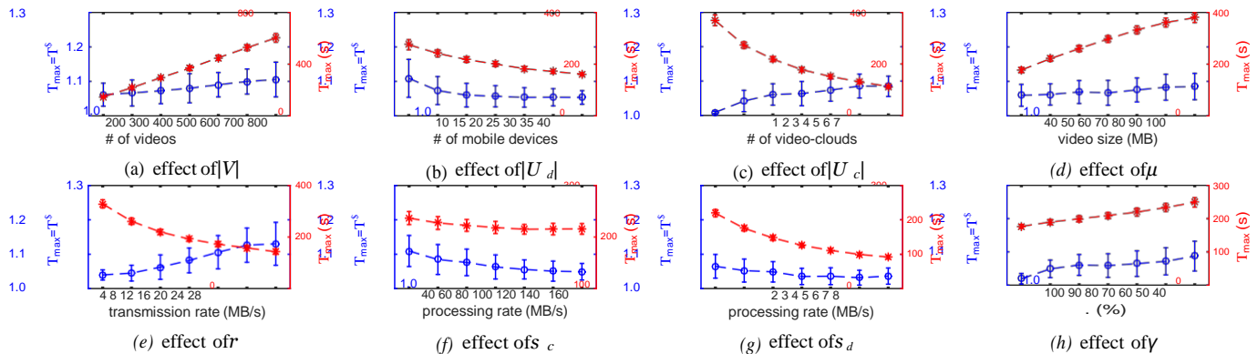
Fig. 5: Comparison between greedy algorithm and optimal solution in terms of T_{max}/T^* and the value of T_{max} , where the default setting is |V|=300 , |U_d|=20 , |U_c|=3 , \mu=50 MB, \sigma=20 MB, r=12 MB/s, s_d=2 MB/s, s_c=100 MB/s and \gamma=0.6 .
