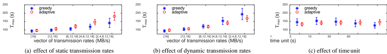
Fig. 7: Comparison between adaptive algorithm and greedy algorithm in terms of T_{max} , where the default setting is V=|100, U|_d=10, U|_c=2|, \mu=50MB, \sigma=20MB, s_d=2MB/s, s_c=100MB/s, \gamma=0.6, t=5s, \text{ and } R=[4,8,12,16] .
