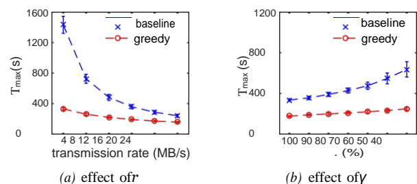
Fig. 6: Comparison between greedy algorithm and baseline in terms of T_{max} , where the default setting is |V|=300 , |U_d|=20 , |U_c|=3 , \mu=50 MB, \sigma=20 MB, r=12 MB/s, s_d=2 MB/s, s_c=100 MB/s and \gamma=0.6 .
