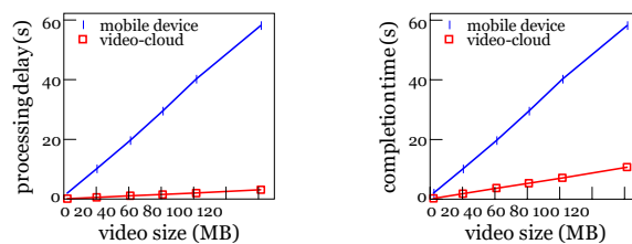
Fig. 4: Processing delay and completion time of videos with different sizes for mobile device and video-cloud, where videos have the resolution 1920x1080, bit rate 16Mbps, frame rate 30fps, and the transmission rate between mobile device and video-cloud is 16Mbps.
