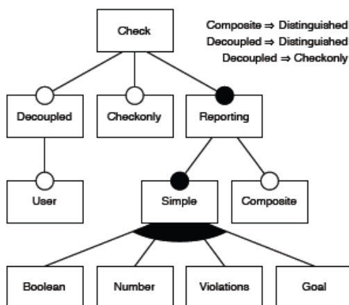
Fig. 11. Check features.
