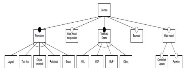
Fig. 8. Domain features.
