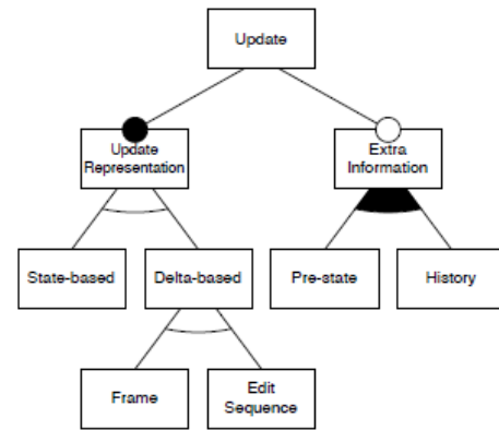
Fig.10. Update features.
