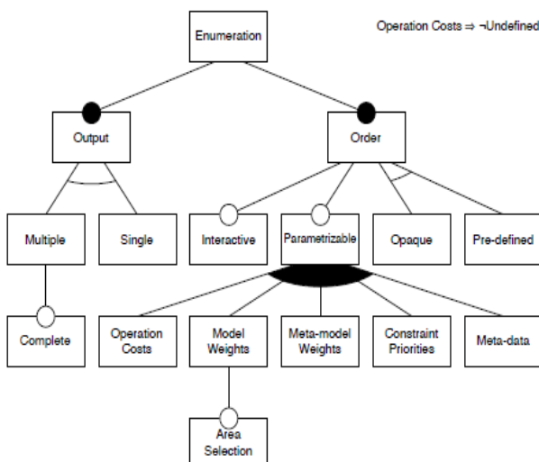
Fig. 13. Repair update enumeration features.
