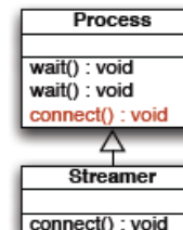
(b) Operation connect created.
