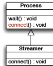
(a) Operation wait renamed.
