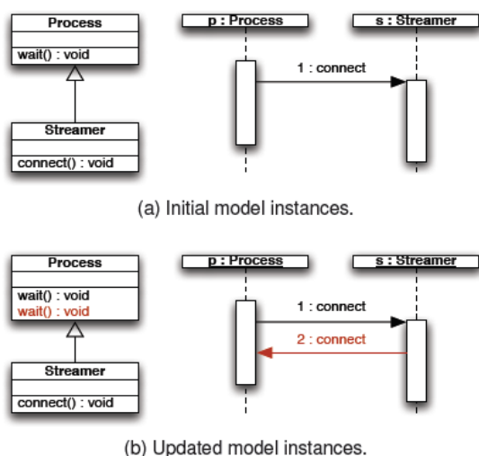
Fig. 3. Inconsistency between the diagrams.
