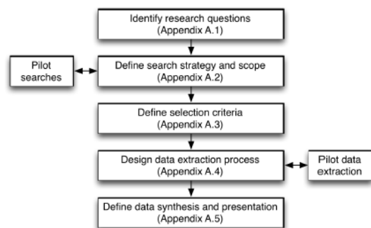
Fig.6. Protocol development process (adapted from [34]).
