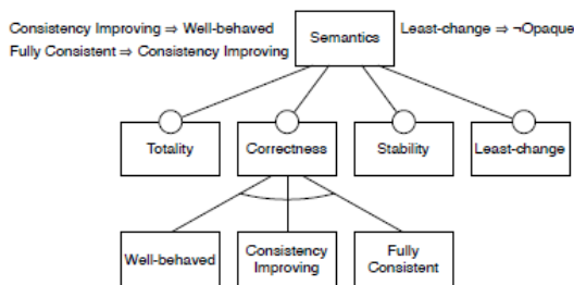
Fig. 14. Repair semantics features.
