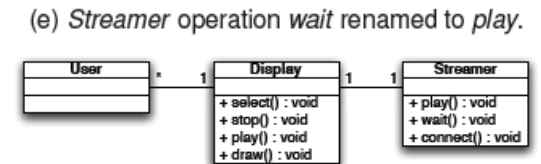
Fig. 16. Model repair update alternatives generated by Echo.
