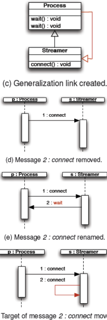
Fig. 4. Possible repair updates for the inconsistency between the diagrams.
