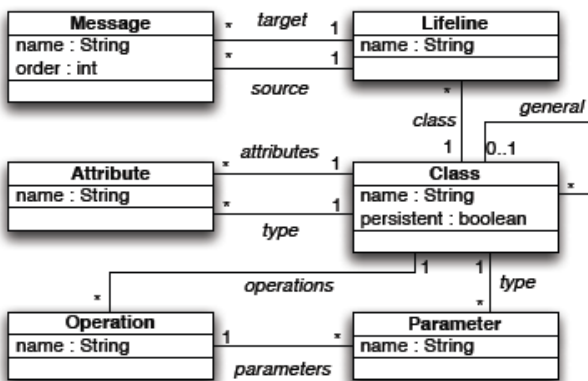
Fig. 1. Simplified meta-model for class and sequence diagrams.
