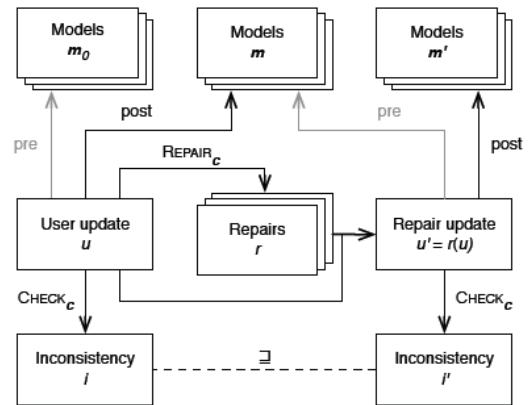
Fig. 5. Generic scheme for model repair.
