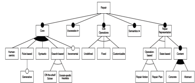
Fig. 12. Repair features.
