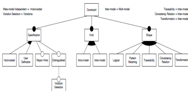
Fig. 9. Constraint features.
