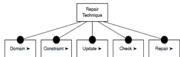
Fig. 7. Model repair features.
