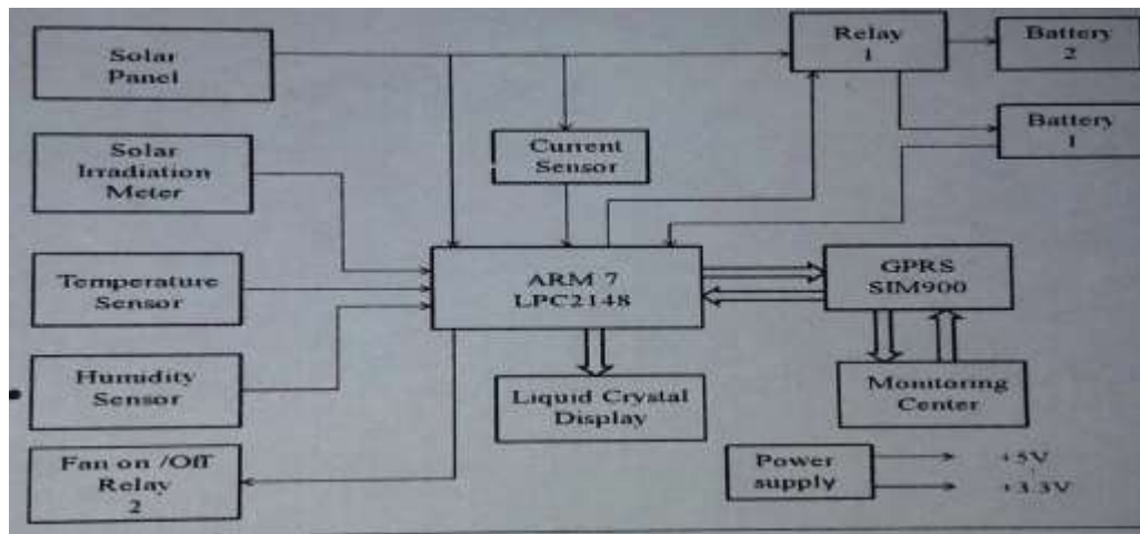
Fig.1 block diagram of solar power monitoring system
