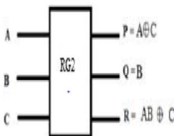
Figure 3.Reversible gate 2
