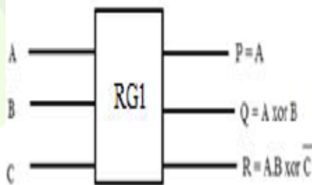
Figure 2. Reversible gate1
