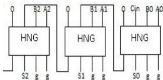
Figure 8. Ripple carry adder
