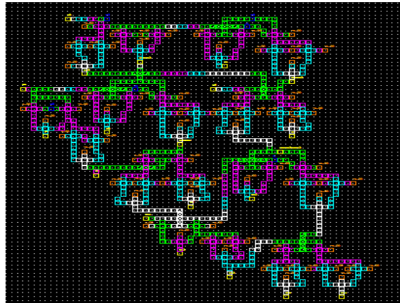
Figure 16. QCA layout for the Logic unit
