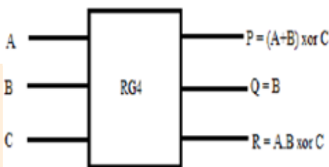
Figure 5. Reversible gate4
