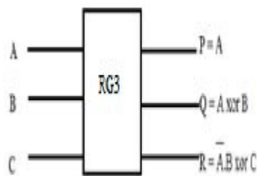
Figure 4. Reversible gate3
