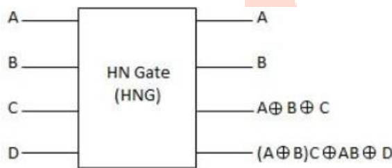
Figure 6. HN gate
