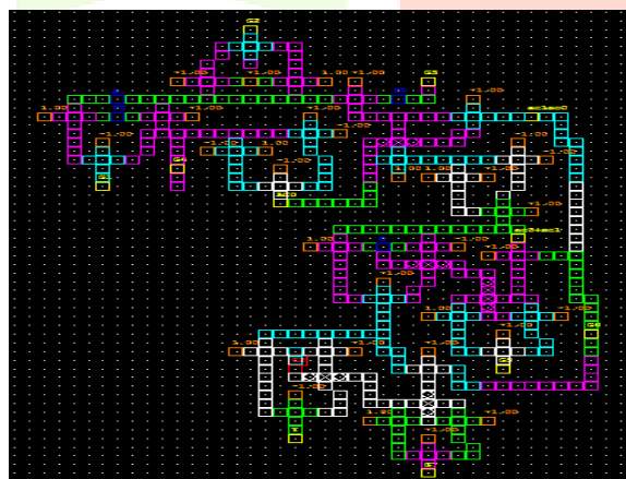
Figure 18. QCA layout for the Arithmetic unit.
