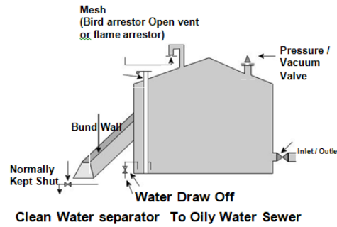
Fig. 2.1 Fixed Roof Tank
