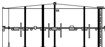
Fig. 2.3 Internal Floating roof Tank.
