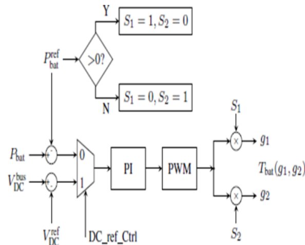
Fig. 4. Battery charging/discharging controller.
