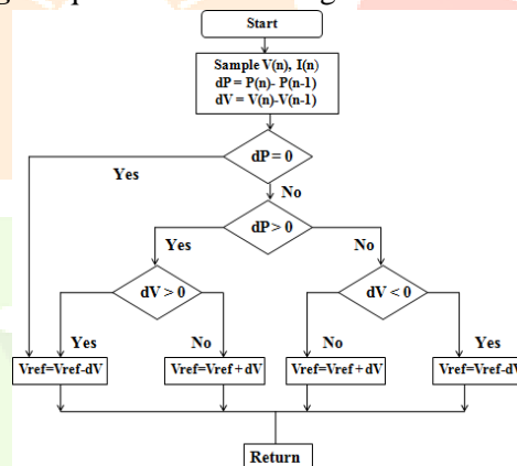
Fig.3 Flow chart of perturb and observe
