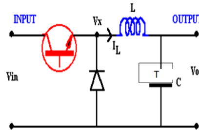
Fig 4 Buck Converter
