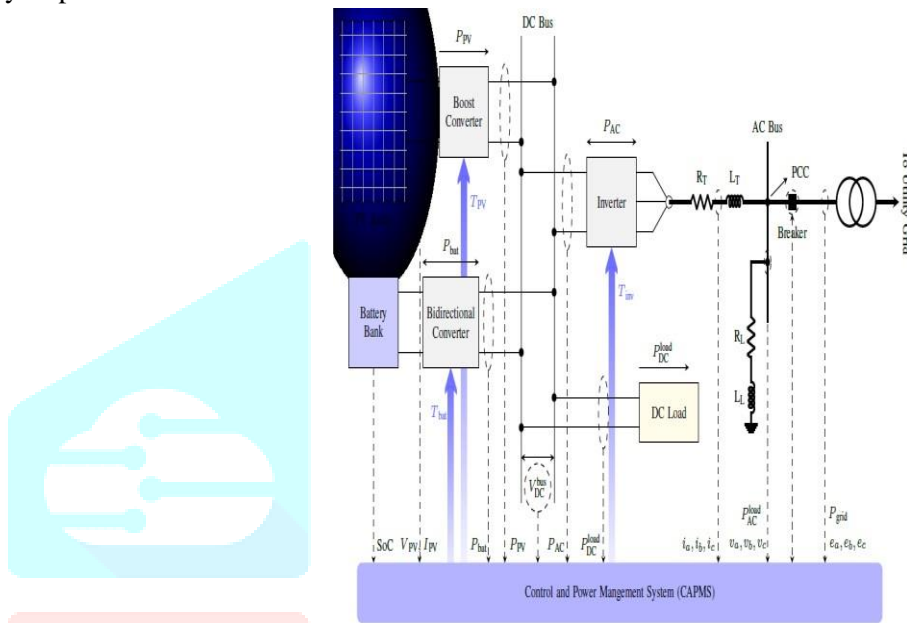
Fig. 1. The proposed control and power management system (CAPMS) for PV-battery-based hybrid microgrids.
