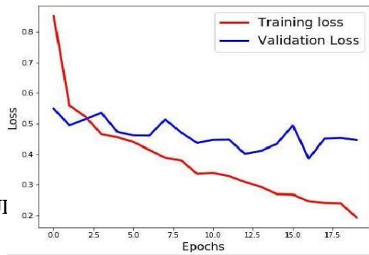
Fig. 3. Training and Validation loss
