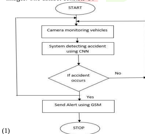
Fig. 1. Working of the System
