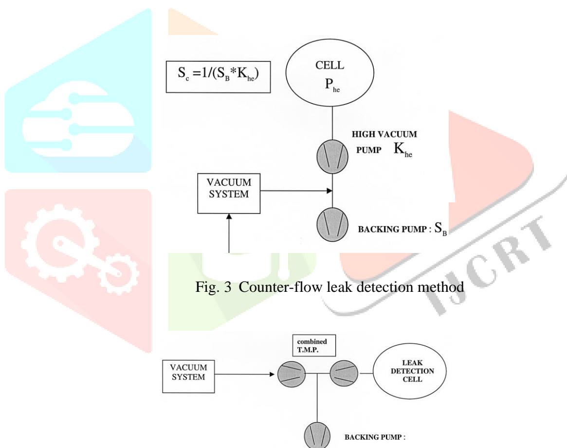
Fig. 4 Combined turbo-molecular-pump leak detector
