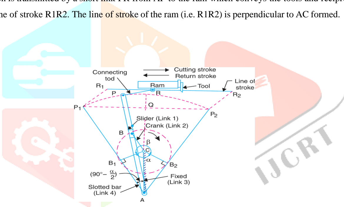
Fig. 1.1 Crank and slotted lever quick return motion mechanism
