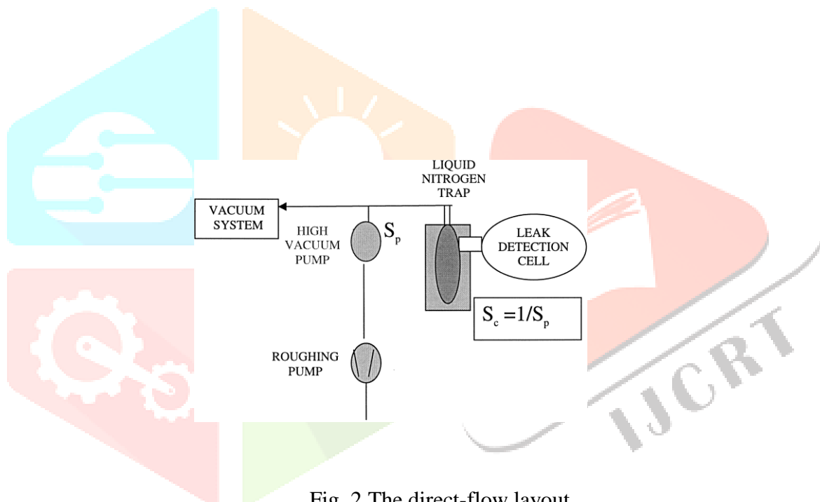
Fig. 2 The direct-flow layout
