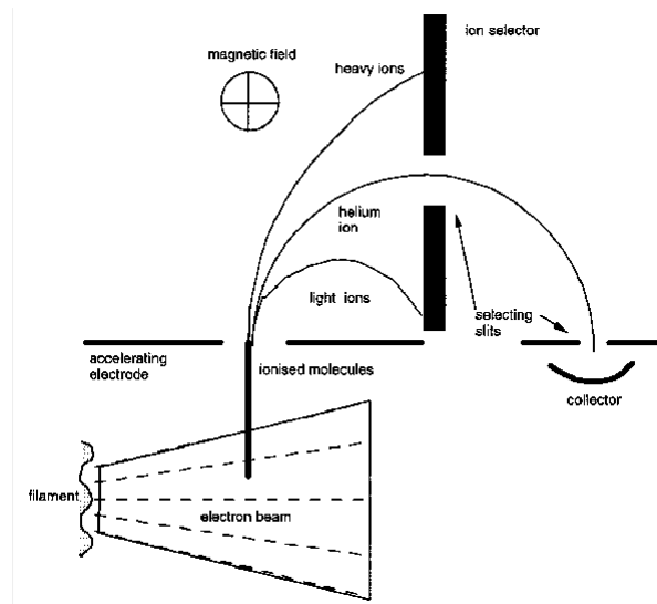
Fig. 1 Schematic layout of a leak detection cell.
