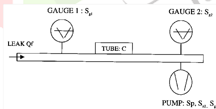
Fig. 7 Leak detection with pressure gauges
