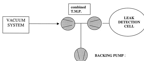
Fig. 4 Combined turbo-molecular-pump leak detector
