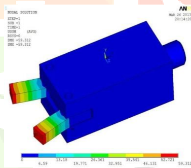
Fig.7 Deformed shape
