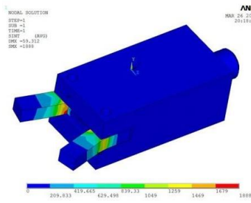
Fig.8 Stress intensity
