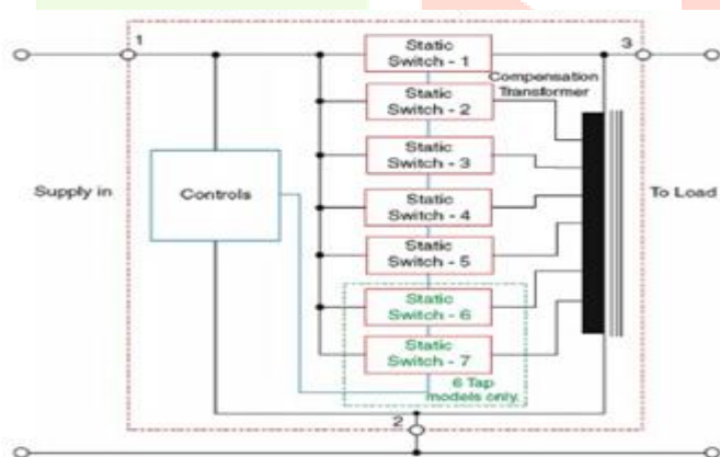
Fig. 1.4 Block Diagram of voltage drop Proofing Transformer
