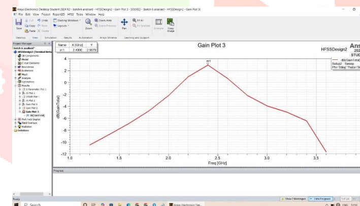
(c) Gain at 2.4 GHz
