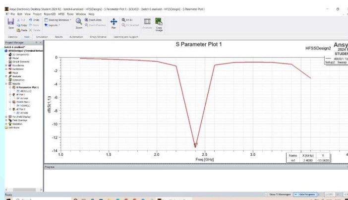
Figure 10: S-parameter at 2.4 GHz
