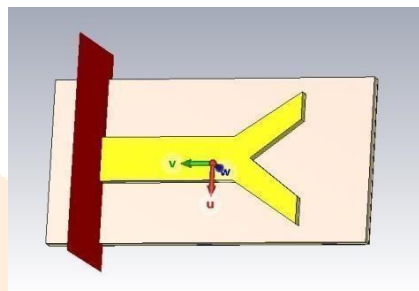
Figure 5: Y-slot Patch Antenna
