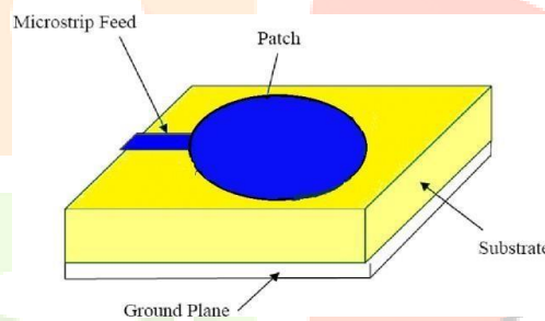
Figure 2: Circular Patch Antenna
