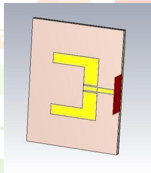
Figure 6: U-slot Patch Antenna
