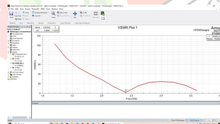
Figure 11: VSWR at 2.4 GHz
