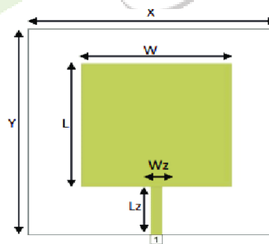
Figure 3: Square Patch Antenna
