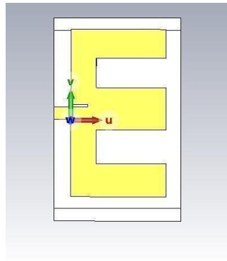
Figure 4: E-slot Patch Antenna
