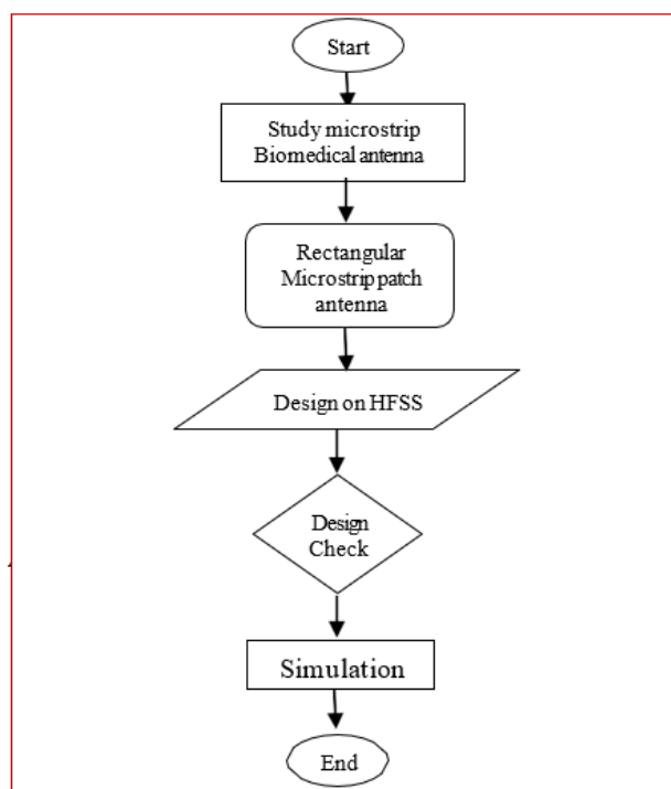
Figure 7: Methodology
