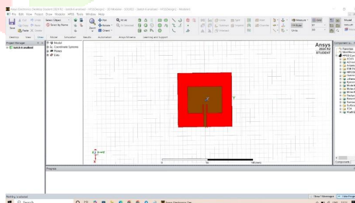
Figure 8: Rectangular Microstrip Patch Antenna
