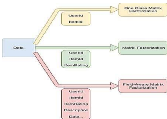
Fig. 2 Matrix factorization techniques available in ML.NET
